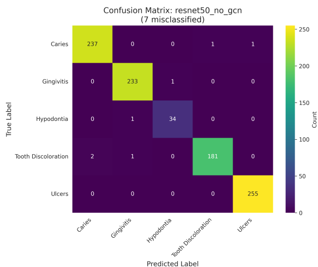
(n) ResNet50 (No GCN)
