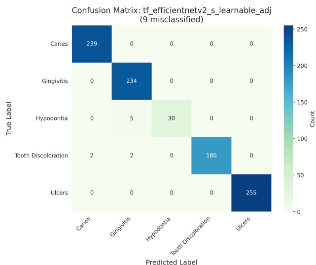
(r) EfficientNetV2-S (Learnable adjacency)
