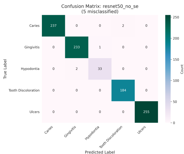
(p) ResNet50 (No SE)
