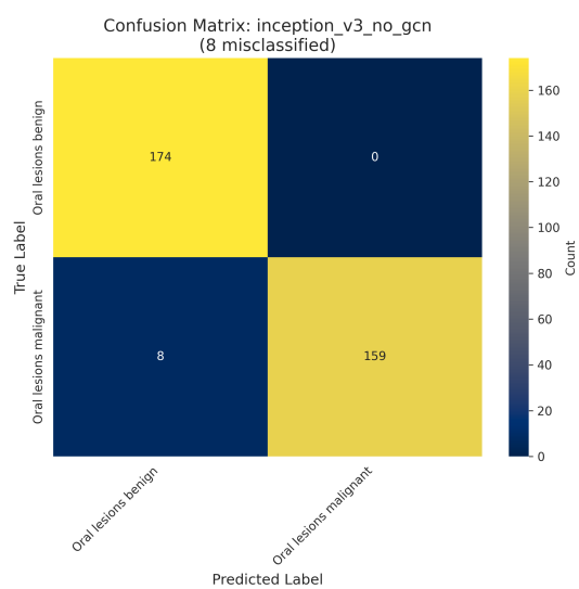
(i) Inception-V3 (No GCN)
