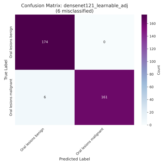
(c) DenseNet121 (Learnable adjacency)
