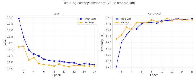
(k) DenseNet121 (Learnable adjacency)
