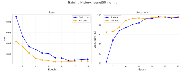
(m) ResNet50 (No MT)
