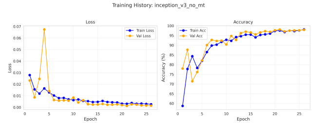
(h) Inception-V3 (No MT)
