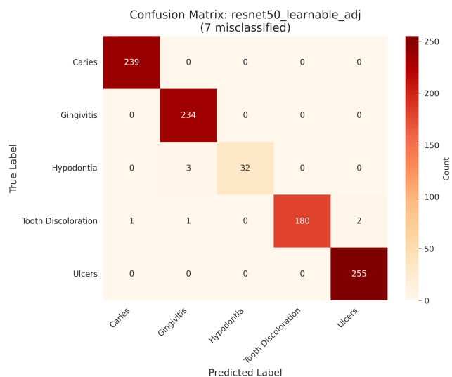
(m) ResNet50 (Learnable adjacency)
