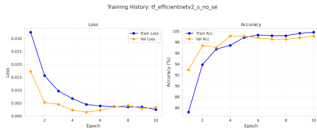
(s) EfficientNetV2-S (No SE)
