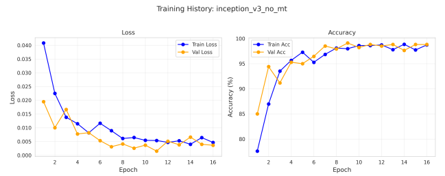
(r) Inception-V3 (No MT)
