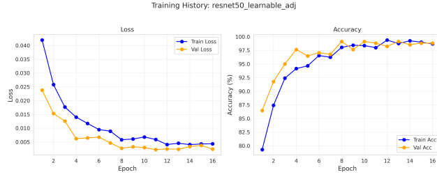
(k) ResNet50 (Learnable adjacency)
