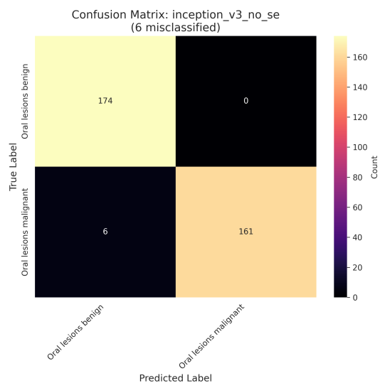
(k) Inception-V3 (No SE)
