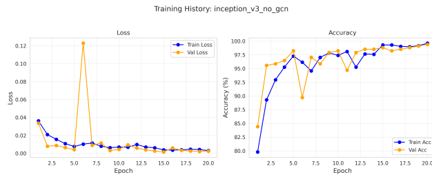
(q) Inception-V3 (No GCN)
