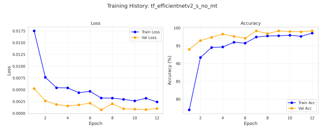
(h) EfficientNetV2-S (No MT)
