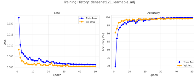
(a) DenseNet121 (Learnable adjacency)
