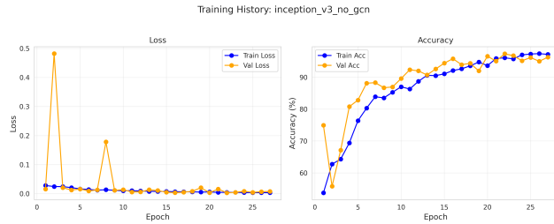
(g) Inception-V3 (No GCN)
