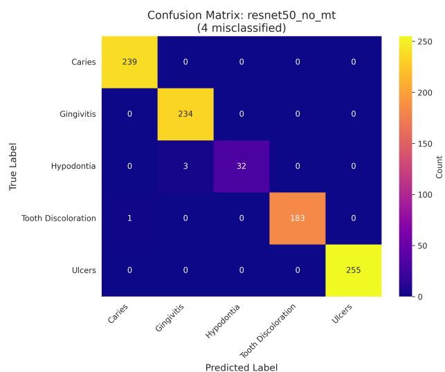
(o) ResNet50 (No MT)
